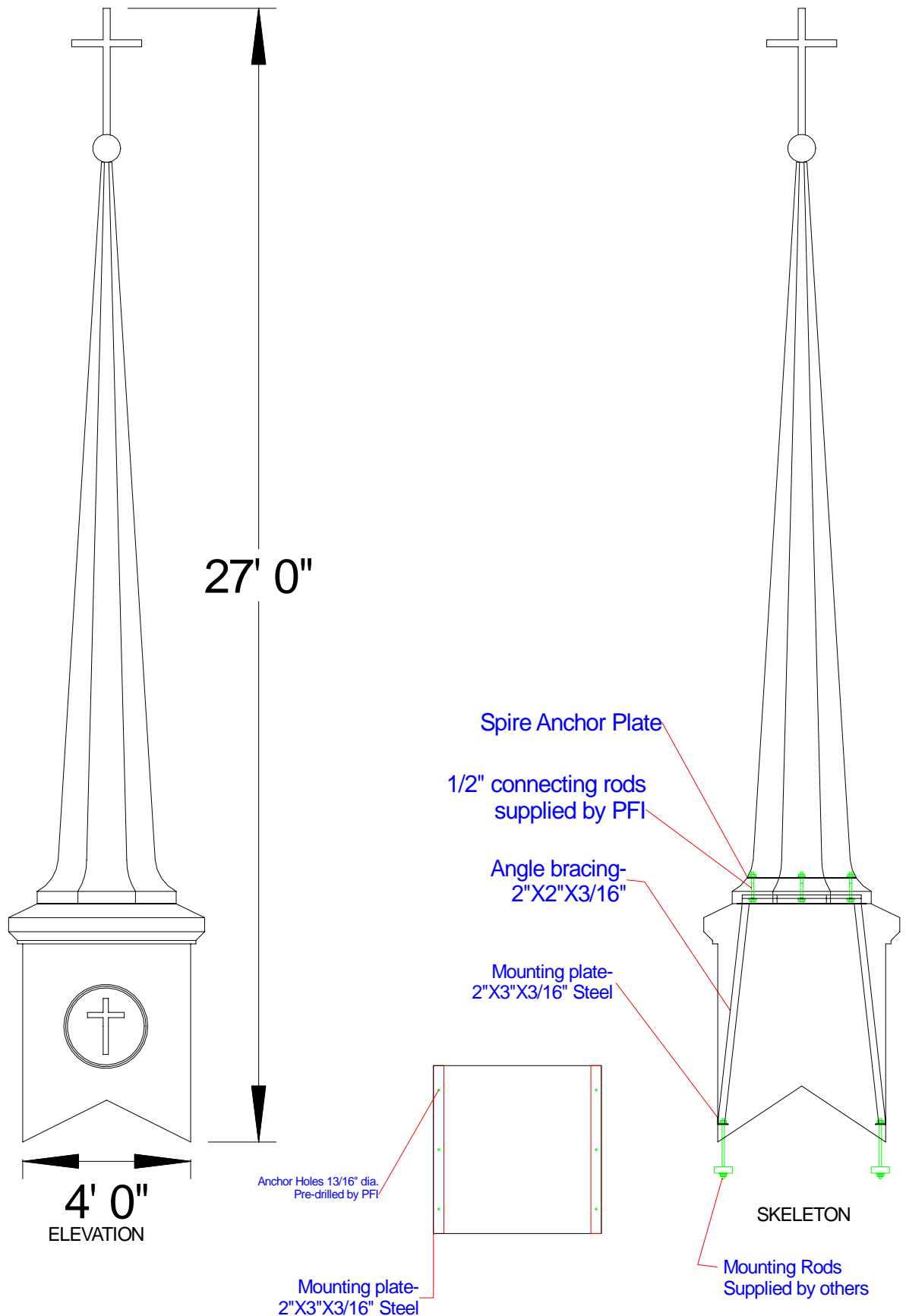
MOUNTING DETAIL
